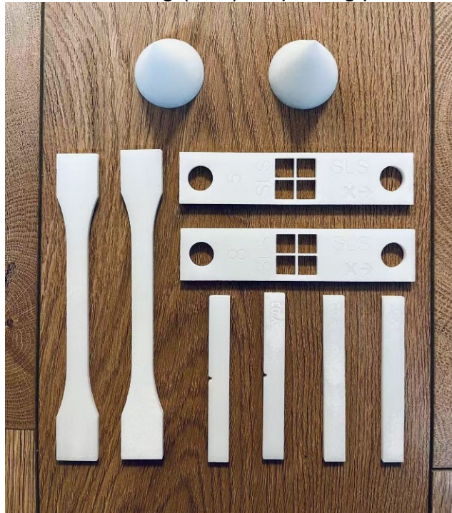
Samples made from Plexint™ CPLA through SLS platforms
